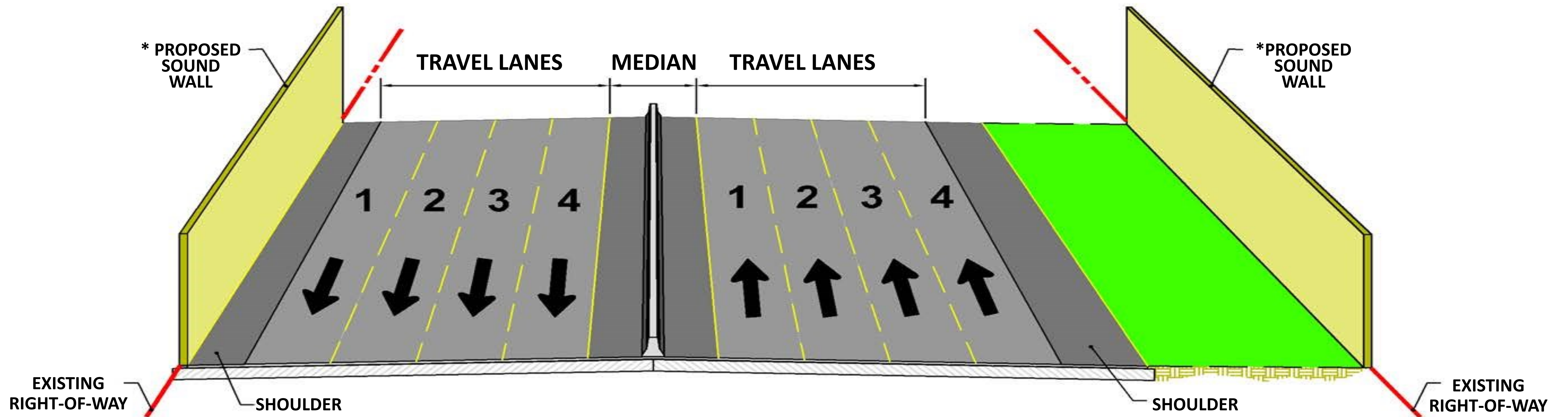
BASE CONCEPT CROSS-SECTION
